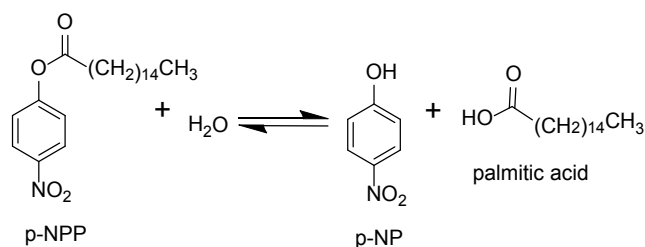
Fig. 1. The hydrolysis of p-nitrophenyl palmitate Investigation of effective factors on enzyme activity
