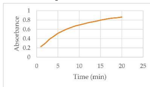
Fig. 2. The absorbance over time of p-nitrophenol from the hydrolysis of the p-nitrophenyl palmitate substrate.
